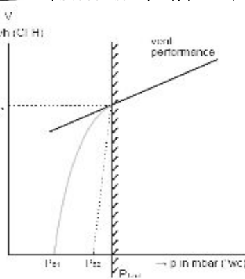
Figure 1: PROTEGO VD/SV1
